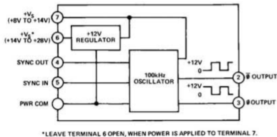
Figure 12. Model 281 Block Diagram
