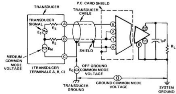
Figure 3. Transducer – Amplifier Interface
