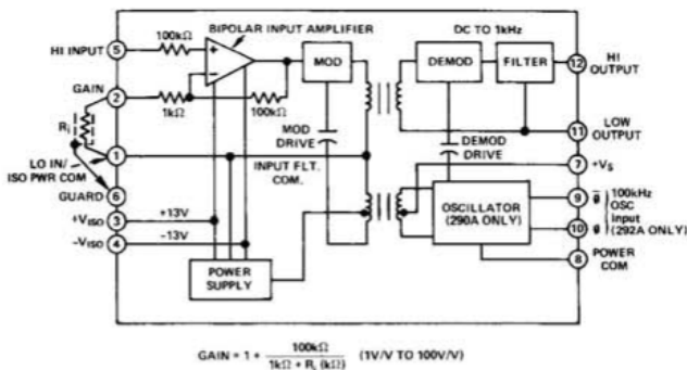
Figure 2. Block Diagram – Models 290A and 292A
