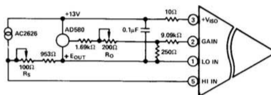
Figure 16. Isolated Temperature Measurements
