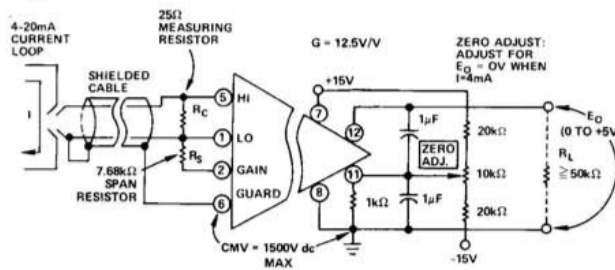
Figure 17. Isolated Analog Interface; 4 to 20mA is Converted to 0 to +5V at the Output, with Up to ±1500V of Isolation
